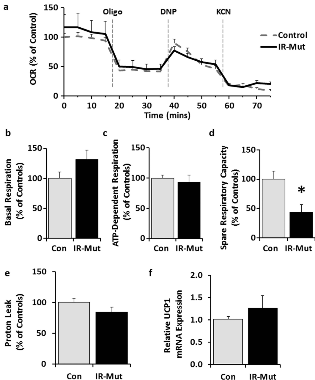
Figure 2. Decreased spare respiratory capacity in IR-Mut iPSC. (a) Bioenergetic profile for oxygen consumption rate (OCR) of control and IR-Mut iPSC assessed at baseline and following sequential addition of oligomycin (10 \mu g/ml), DNP (10 \mu M) and KCN (50 nM). OCR was analysed at 5-minute intervals and normalised by DNA ( n = 3 ). (b) Basal OCR was calculated from the last measurement before oligomycin addition minus non-mitochondrial respiration. (c) ADP-dependent respiration calculated from last measurement before oligomycin minus minimum measurement after oligomycin. (d) Spare respiratory capacity calculated from maximum measurement after DNP minus last measurement before oligomycin. (e) Proton leak calculated from minimum measurement after oligomycin minus non-mitochondrial respiration. (f) Relative mRNA expression of uncoupling protein 1, as assessed by qRT-PCR. Data are normalised to 36B4 and expressed relative to control ( n = 3 ). * p < 0.05 for IR-Mut vs. control.
