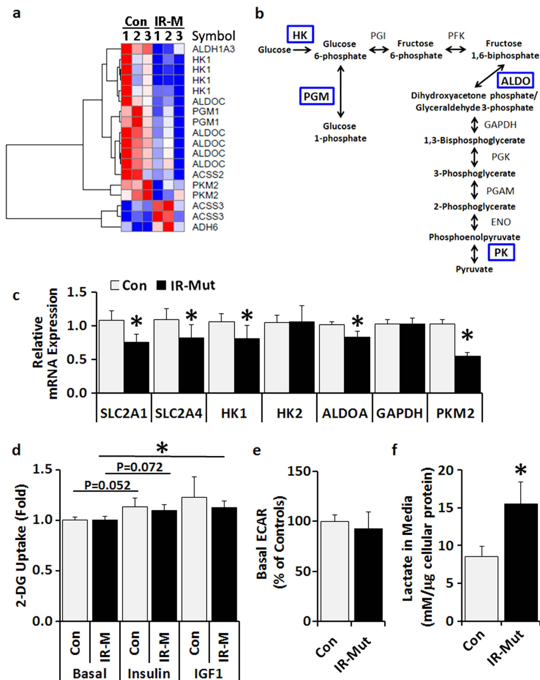
Figure 4. IR-Mut iPSC have increased extracellular lactate. (a) Heat map of differentially expressed genes (nominal p < 0.05 ) related to glucose metabolism based on KEGG glycolysis/gluconeogenesis gene set, as determined by microarray analysis, with red indicating increased expression and blue indicating decreased expression. (b) Glycolysis pathway schematic of enzymes with significantly decreased mRNA expression in IR-Mut iPSC (indicated in blue). (c) Relative mRNA expression of glucose metabolism genes, as assessed by qRT-PCR. Data are normalised to 36B4 and expressed relative to control cells ( n = 3 ). (d) [ ^3\text{H} ]-2-deoxyglucose uptake was assessed at baseline and in response to 100 nM insulin and 10 nM IGF1. Data are expressed relative to basal control values ( n = 4 ). (e) Basal extracellular acidification rate (ECAR) in control and IR-Mut iPSC, expressed relative to control and normalised by DNA concentration ( n = 3 ). (f) Lactate concentrations in conditioned medium at 0 and 4 hours after addition of fresh media and normalised to cellular protein content ( n = 4 ). *indicates p < 0.05 for IR-Mut vs. control.
